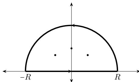
Figure 4: Contour in the upper half-plane, with the three points denoting the three simple poles of f(z) in the upper half-plane.
